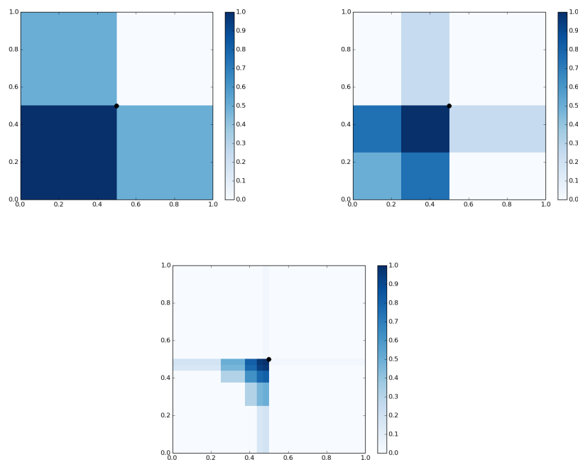
Fig. 3 Representations of f_1 , f_2 and f_5 in [0, 1]^2 .
